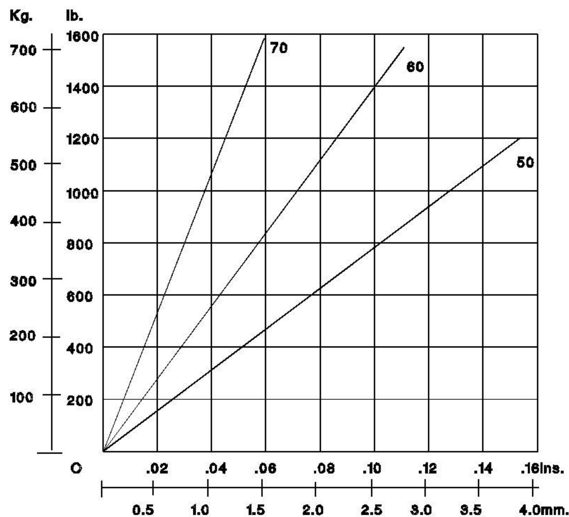
GRAPH : STATIC LOAD VS. DEFLECTION
