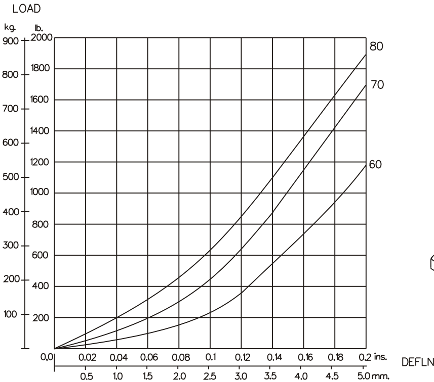
GRAPH 1 : STATIC AXIAL(VERTICAL) LOAD VS. DEFLECTION
