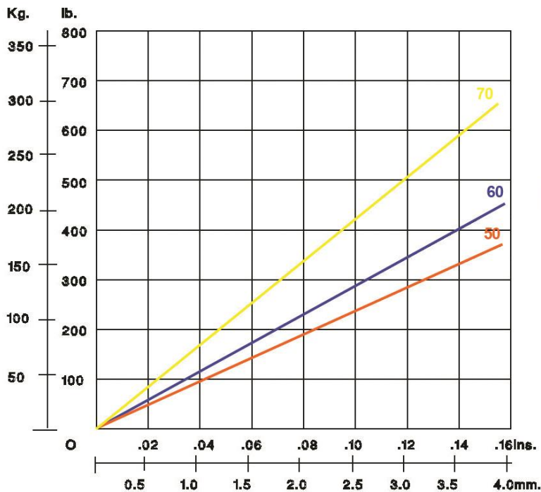
GRAPH : STATIC LOAD VS. DEFLECTION
